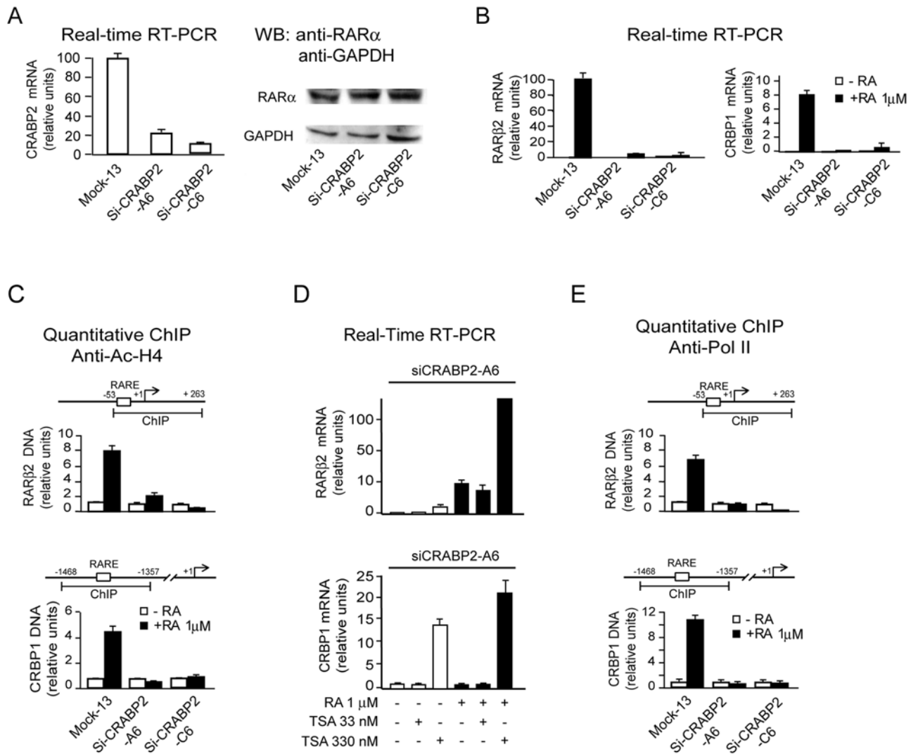
Figure 2. Evidence of chromatin repression at RA-responsive genes downstream of RARα consequent to CRABP2 knock-down. (A) The HME1-derived stable clones Si-CRABP2-A6 and Si-CRABP2-C6, carrying two distinct CRABP2 -targeting shRNA sequences ( CRABP2 -A and CRABP2 -C, respectively), display a significant decrease in CRABP2 transcript relative to the control clone Mock-13 (left). The level of RARα expression is similar in Si-CRABP2-A6, Si-CRABP2-C6 and the control clone Mock13 (right). (B) Both RARβ2 (left) and CRBP1 (right) are significantly less inducible by RA (72 h) in Si-CRABP2-A6 and Si-CRABP2-C6 clones relative to the control Mock13 clone. (C) qChIP analysis with anti-acetyl histone H4 (Ac-H4) showing that RARβ2 (top) and CRBP1 (bottom) chromatin of both Si-CRABP2-A6 and Si-CRABP2-C6 is marked by H4 hypoacetylation at the RARE-containing regulatory regions relative to the control clone Mock-13. (D) RA-induced RARβ2 (top) and CRBP1 (bottom) transcription can be restored in Si-CRABP2-A6 cells by treatment with the HDAC inhibitor TSA. (E) qChIP with anti-Polymerase II (Pol II) showing decreased occupancy of Pol II at the RARE-containing regions of both RARβ2 (top) and CRBP1 (bottom) in Si-CRABP2-A6 and Si-CRABP2-C6. doi:10.1371/journal.pone.0004305.g002
