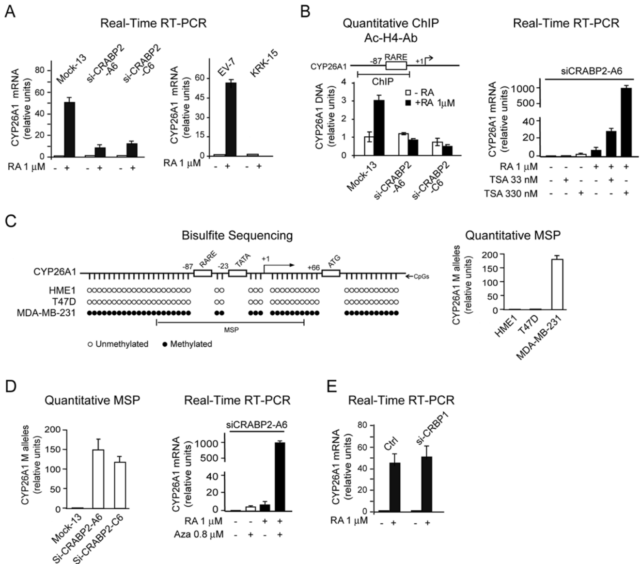
Figure 5. Derangement of CRABP2 function exerts a chromatin repression effect branching downstream of RARβ2. (A) RA-induced transcription of CYP26A1 is significantly downregulated in both HME1 cells knocked down for CRABP2 (Si-CRABP2-A6 and Si-CRABP2-C6 clones, left), and HME1 cells carrying the CRABP2-KRK mutant (KRK-15 clone, right) relative to control cells (Mock 13 and EV7 clones, respectively). (B) qChIP analysis with anti-acetyl histone H4 showing that CYP26A1 chromatin in Si-CRABP2-A6 and Si-CRABP2-C6 clones is marked by a significant H4 hypoacetylation of a region encompassing the CYP26A1 proximal RARE (left). RA-induced CYP16A1 transcription can be restored in Si-CRABP2-A6 by treatment with the HDAC inhibitor TSA for 72 h (right). (C) Bisulfite sequencing showing that HME1, like the CYP26A1 -positive cell line T47D, is unmethylated in the proximal RARE-containing CpG island, while the CYP26A1 -negative cell line MDA-MB-231 is fully methylated (left). Quantitative MSP with primers recognizing only methylated (M) alleles can detect methylation in MDA-MB-231, but not in T47D or HME1 cells (right). (D) Quantitative MSP analysis showing hypermethylation of CYP2A1 proximal CpG island in Si-CRABP2-A6 and Si-CRABP2-C6 clones (left). RA-induced CYP26A1 transcription can be efficiently restored in Si-CRABP2-A6 cells by treatment with the demethylating agent 5-Aza (right). (E) CYP26A1 transcription can still be induced by RA in HME1 cells knock down for CRBP1 (Si-CRBP1). Thus, CYP26A1 epigenetic downregulation is not consequent to CRBP1 epigenetic silencing. doi:10.1371/journal.pone.0004305.g005
